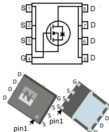
DFN5*6
